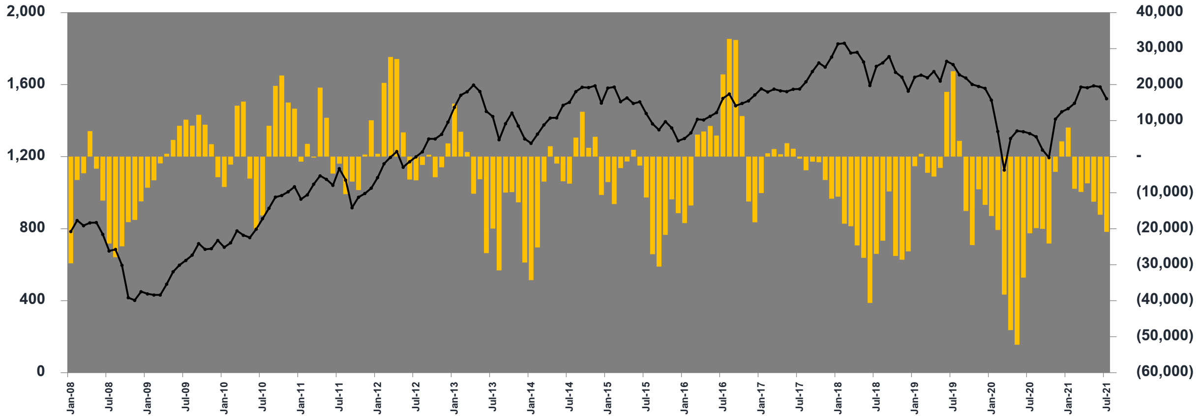
Foreign net buy and SET Index
